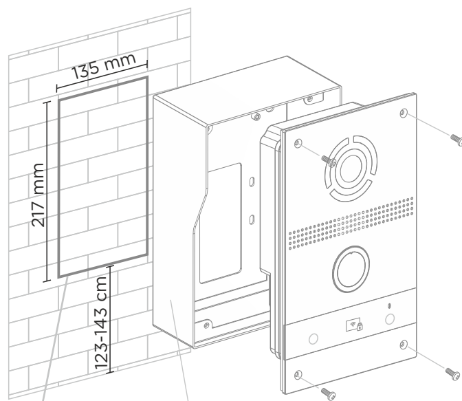
Mounting area
